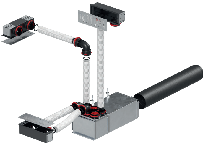
RapidLock® Connection System
